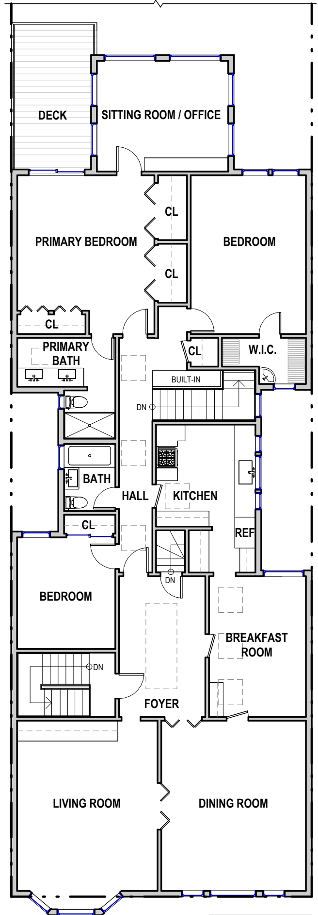
LEVEL 2
